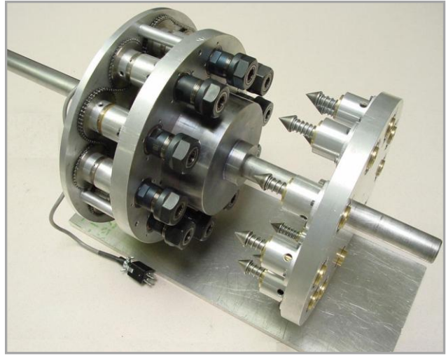
12 Spindle Carousel - with Tailstock
