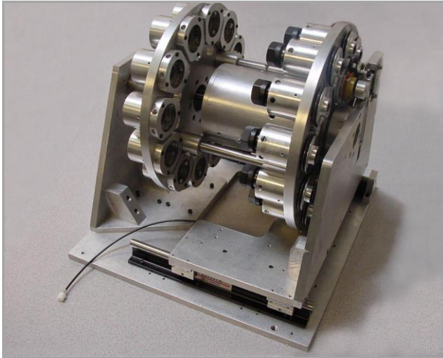
12 Spindle Carousel
