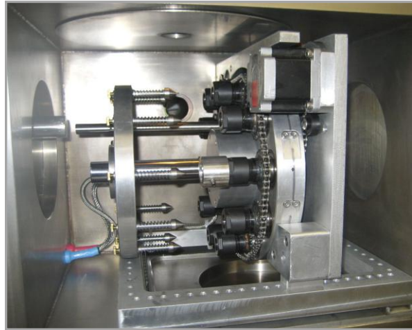
10 Spindle Carousel - Horizontal View with Tailstock
